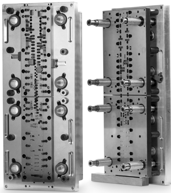
Progressive tool.
